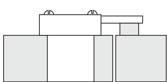
CL10-354 or CL10-355 Bar Strike Shown surface mounted on wood Surface mount on metal also acceptable
